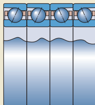
串联后背对背配置 代号后缀QBC
