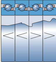
串联背对背 代号后缀QBC
