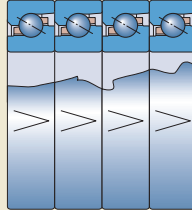
串联 代号后缀QT
